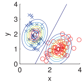
Equal var.
